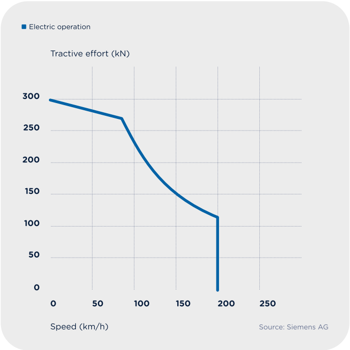
Traction effort diagram for the Vectron AC
